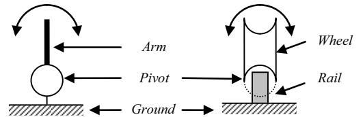
Fig. 4: (a) classical bilateral pivot joint and (b) unilateral pivot joint
