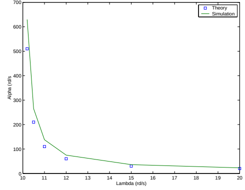
Figure 3: Stability limit
