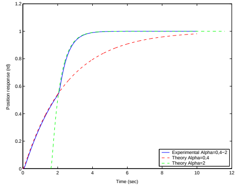
Figure 7: Position response
