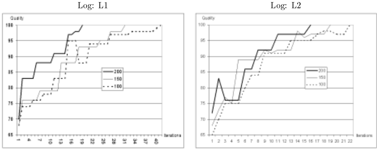
Figure 16: Results quality for each proposed solution
