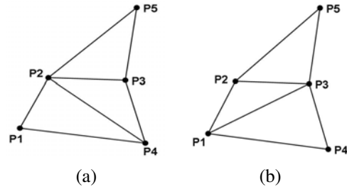
Figure 5: a) Initial triangles, b) Triangles after the embedding.
