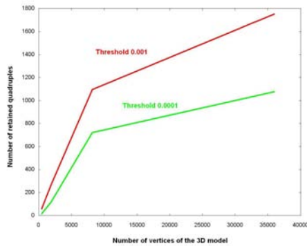
Figure 11: Number of retained quadruples in function of the number of vertices of the 3D model.
