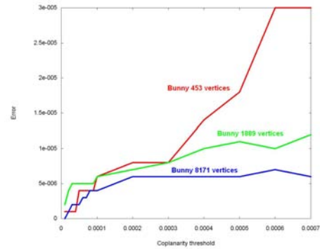
Figure 13: Error in function of coplanarity threshold.
