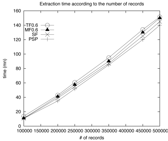
Fig. 6. Runtime according to the number of records in the datasets, minFreq=0.6
