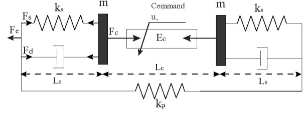
Fig. 2. Macroscopic skeletal muscle model.
