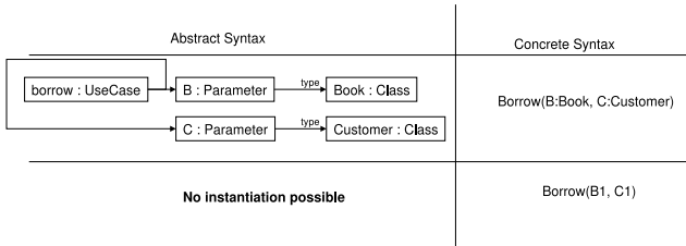
Figure 6. Instantiation issue for use cases
