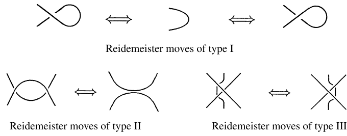
FIGURE 3. Reidemeister moves.
