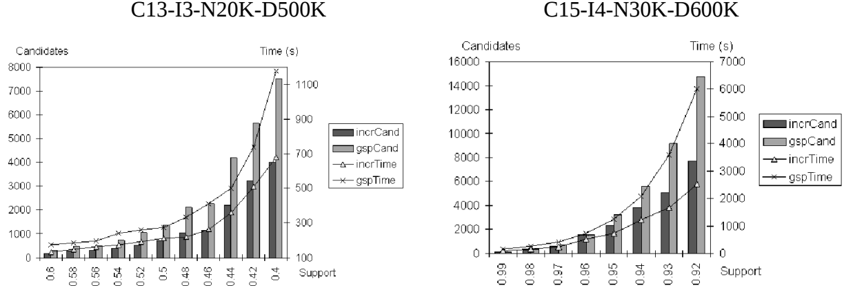
Fig. 12. Candidate sets
