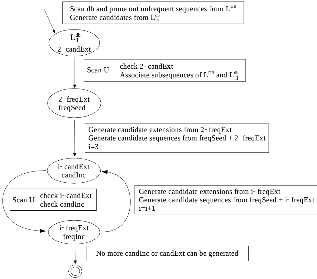
Fig. 7. Processes in the first and j^{\text{th}} iterations of ISE
