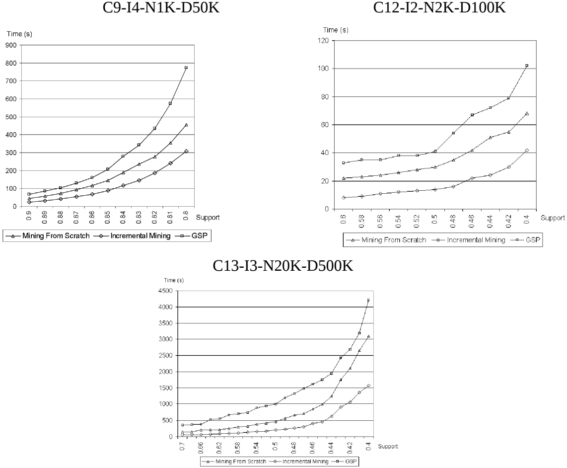
Fig. 8. Execution times
