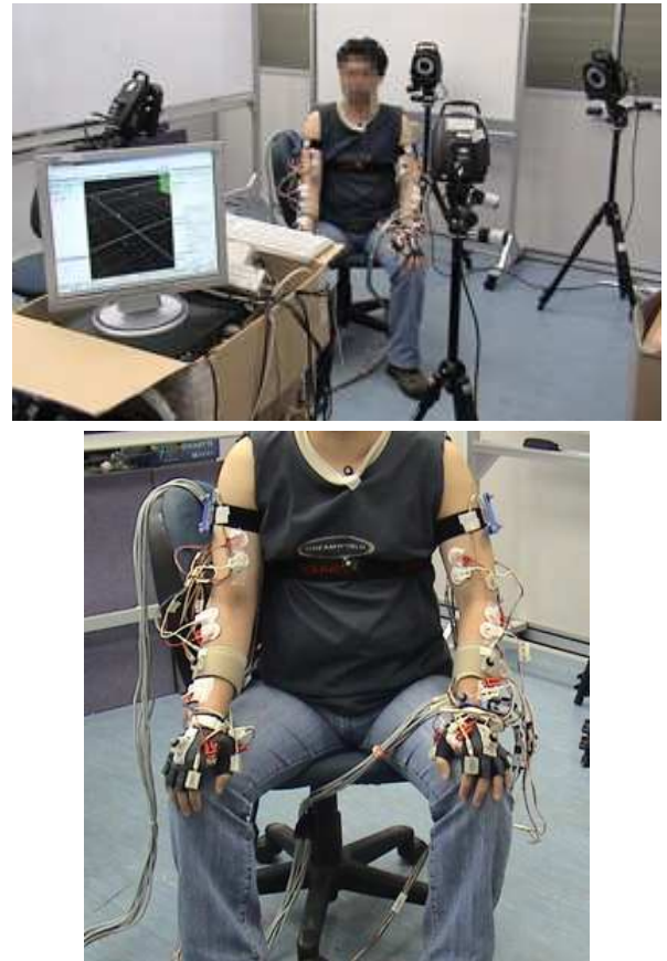
Fig. 2. The whole setup for the sensing system developed.
