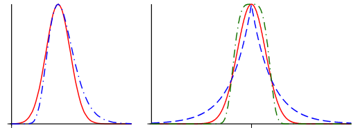
Figure 4: Left: Comparison between Gaussian (continuous line) and Lognormal (dotted line) functions. Right: The generalized Gaussian function: \alpha=1 = Laplace function (dashed line), \alpha=\sqrt{2} = Gaussian function (continuous line) and \alpha=2 (dotted line).
