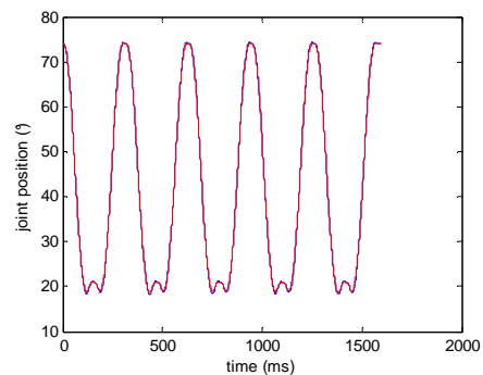
Red: commanded position, blue: measured position Figure 20 : commanded and measured joint positions
