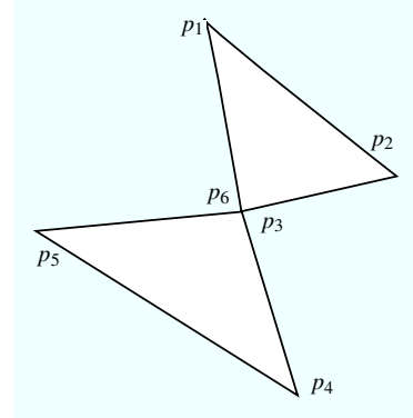
Fig. 4. (b) A nearly polygonal gallery defined by the sequence (p_1, p_2, p_3, p_4, p_5, p_6, p_1) , with p_6 = p_3 .
