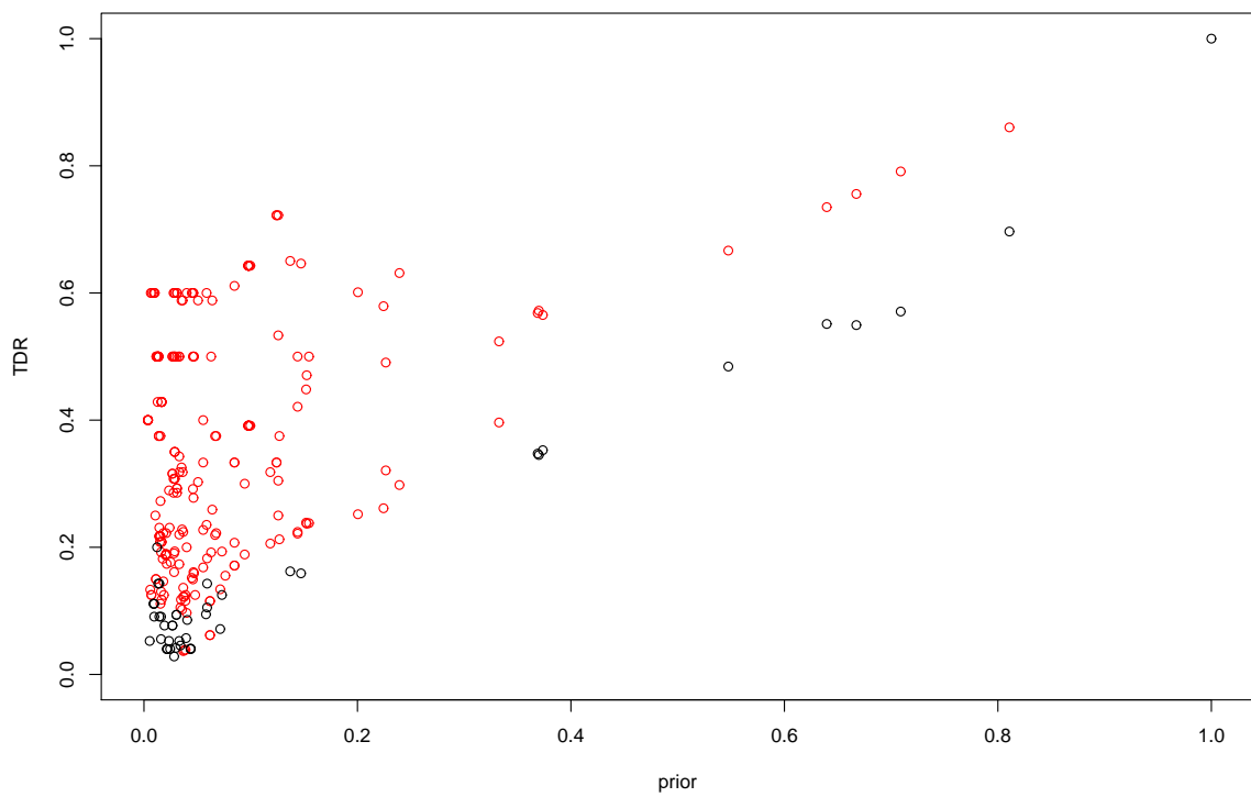
Figure 6 — Gonna performances on the transcriptomic data set published in Bozdech et al. (2003) [27]. TDRs of all BP GO terms where predictions are proposed by Gonna are plotted as a function of the prior probability of the terms. Red and black points indicate significant and non-significant TDRs , respectively.
