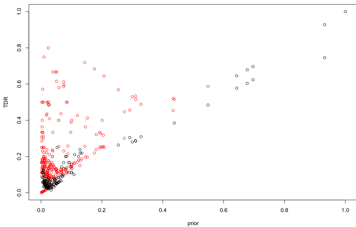
Figure 5 — Gonna performance on yeast. Gonna was applied to the transcriptomic data set published by Spellman et al. (1998) [34] using experimental evidence code annotations only as prior knowledge database. TDRs of all BP GO terms where predictions are proposed by Gonna are plotted as a function of the prior probability of the terms. Red and black points indicate significant and non-significant TDRs , respectively.
