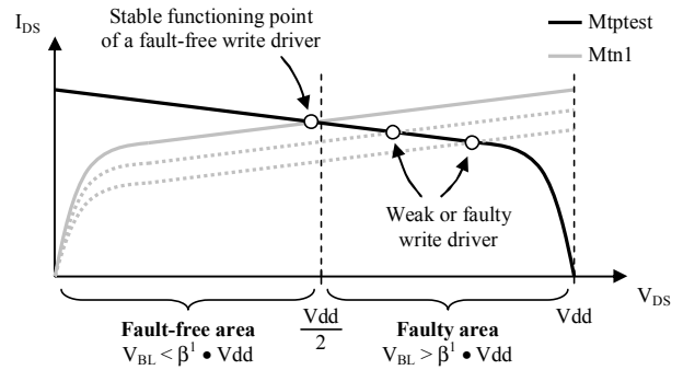
Figure 5: Principle of the diagnosis solution
