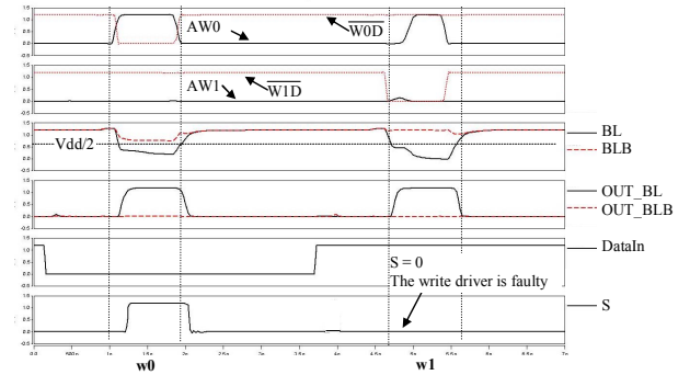
Figure 9: Simulation results of a faulty write driver
