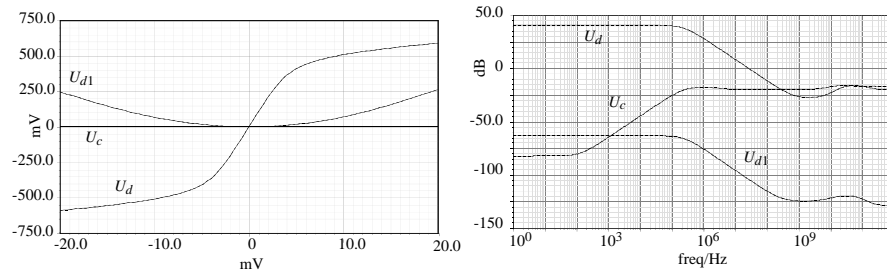
Fig. 13. Simulated static response and frequency response of the preamplifier. U_c stands for the common mode voltage (to be rejected), U_d is the component we want to amplify while U_{d1} is a parasitic differential voltage.
