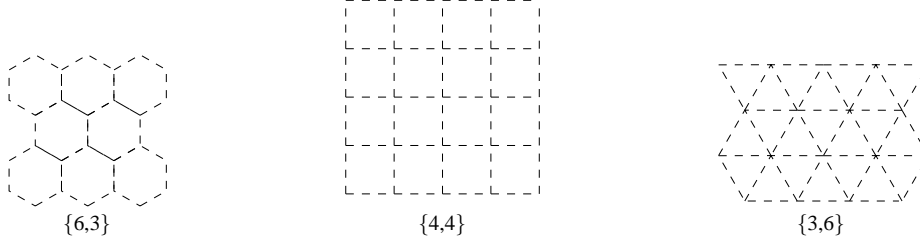
Fig. 3. There are exactly three regular tessellations composed of regular polygons symmetrically tiling the plane.
