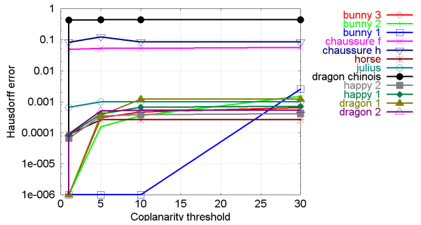
Figure 14: Maximum Hausdorff error in function of coplanarity threshold.
