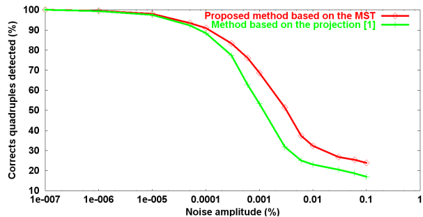
Figure 15: Correct quadruples detected with a threshold S_c = 10^\circ (for the average of the 12 analyzed objects).
