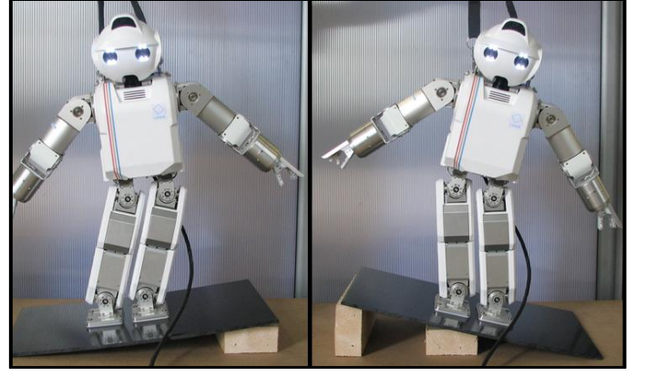
Fig. 13 SESC Modeling used to control CoM Projection on leaning ground
