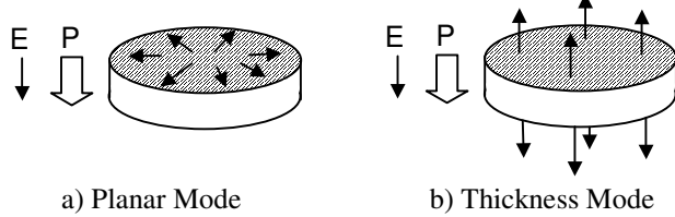
a) Planar Mode b) Thickness Mode Fig. 1: Typical vibration modes of ceramic disks
