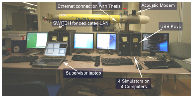
Fig. 5. The Thetis system and the AUV Taipan300
