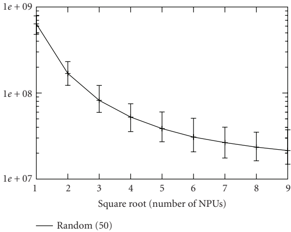
FIGURE 11: Objective function value space for 50 tasks and random mapping.
