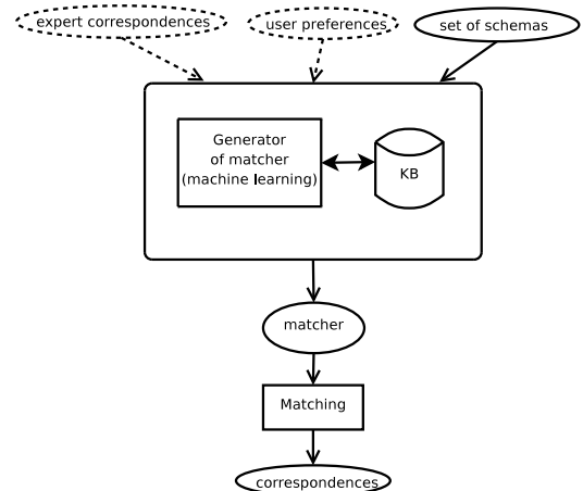
Figure 5: YAM architecture
