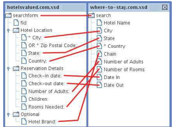
Figure 2: Expert correspondences between the two hotel booking webforms
