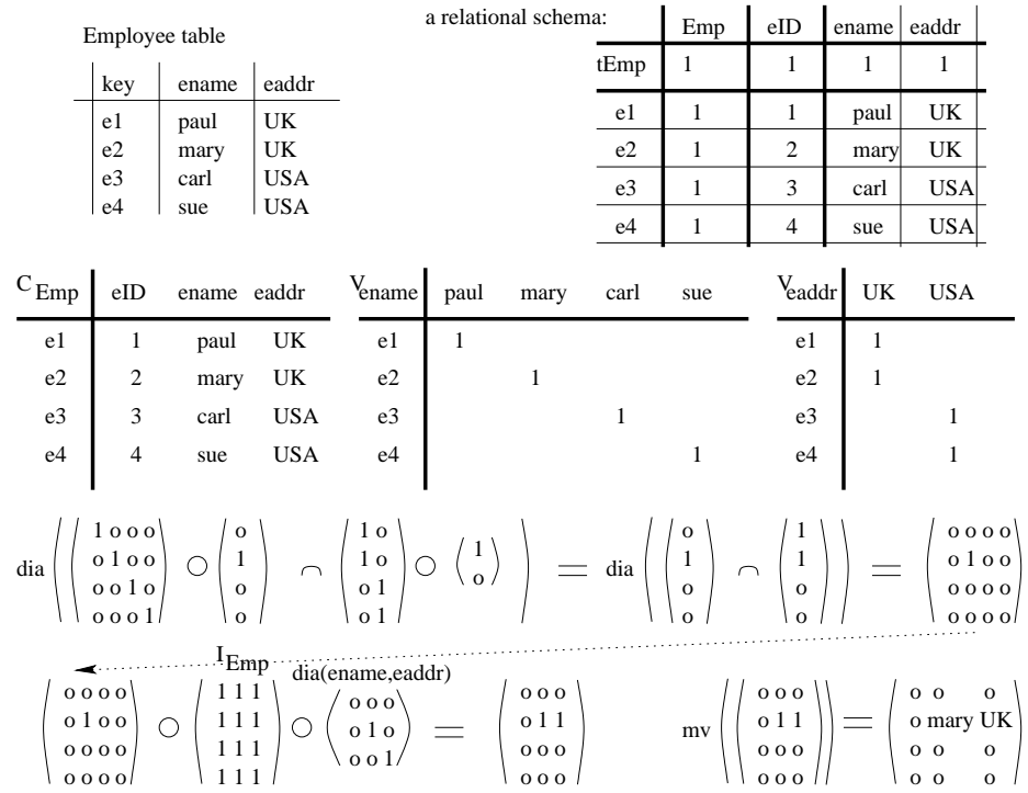
Fig. 6. Calculating \text{dia}((V_{\text{ename}} \circ \text{mary}^d) \cap (V_{\text{eaddr}} \circ \text{UK}^d)) \circ I_{\text{Emp}} \circ \text{dia}(\underline{\text{ename}}^d \cup \underline{\text{eaddr}}^d) or: select ename,eaddr from Emp where ename='mary' and eaddr='UK'
