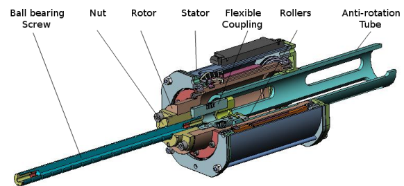
Fig. 8. Cut out section view of the hollow shaft actuator and ball bearing transmission
