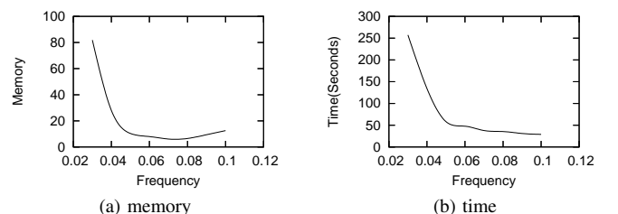
Fig. 3. 1000 transaction and 100 items performances
