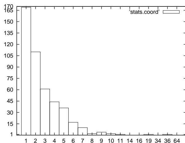
Fig. 5. Outlier distribution
