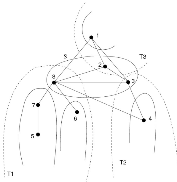
Figure 4. The slices defined by an execution of MCS on a chordal graph. The substars of 1 are \{8\} and \{3, 8\} .
