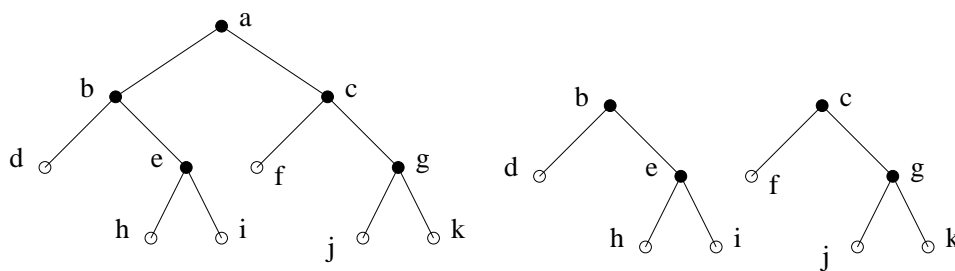
Figure 2. \{a\} is a df -separator.
