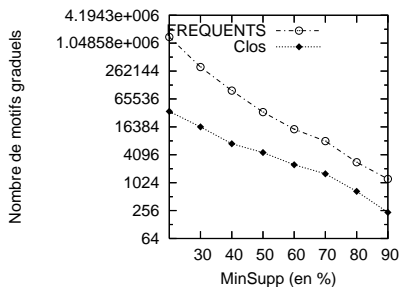
Fig. 4. Number of gradual closed patterns vs frequent with minsup variation
