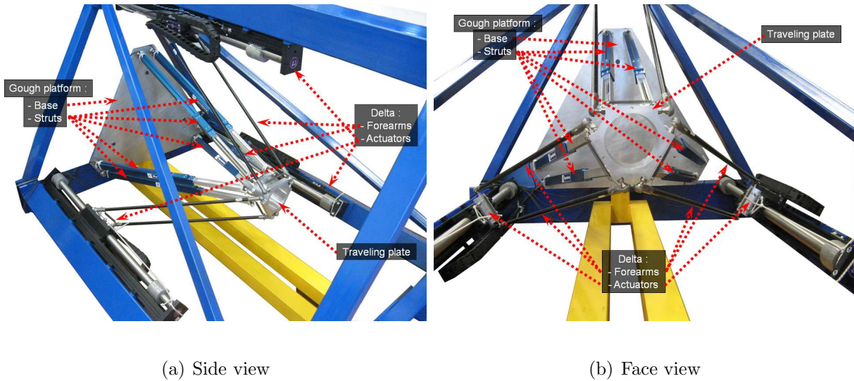
Figure 8: MoM3 Prototype
