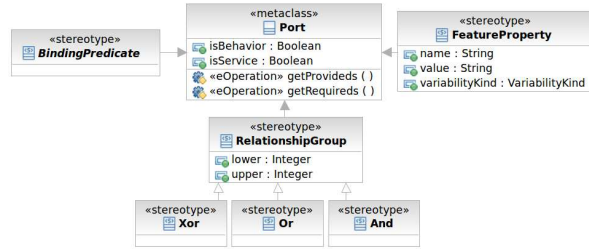
Figure 5 – Meta-classes extensions
