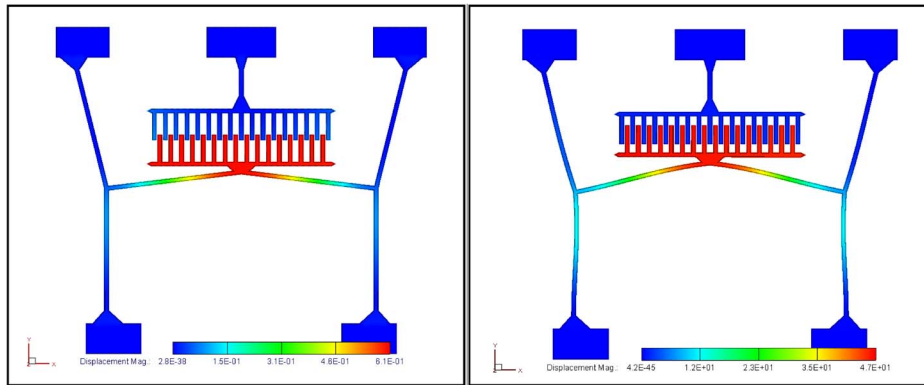
Fig. 7. Coventor simulation through CoSolve: Two results obtained (left) at 298 K and (right) at 500 K.
