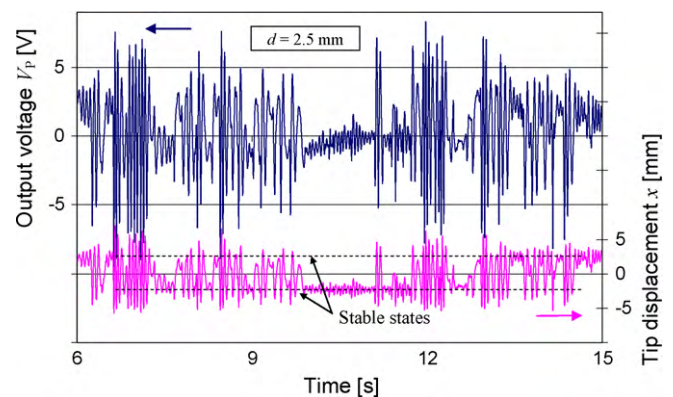
Fig. 12. Output voltage V_p and tip displacement of the piezoelectric converter in a nonlinear behaviour condition, with an acceleration of the input vibrations a_{\text{rms}} = 0.3\ \text{g} .
