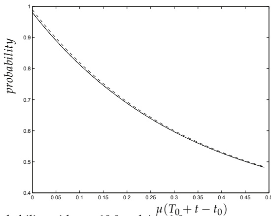
Fig. 4. Existence probability with \gamma = 10.0 and \Delta = 1.0
