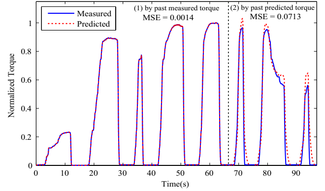
Fig. 7. The measured and predicted torque obtained by eEMG-to-torque model in random test in subject S5. The vertical dotted line is shown to separate the data into two parts. The model was identified by OLS method using the data in the left part. (1) The torque was predicted based on the past measured MAV of eEMG and past measured torque. (2) The torque was predicted based on the past measured MAV of eEMG and past predicted torque, where the prediction was calculated only by eEMG.
