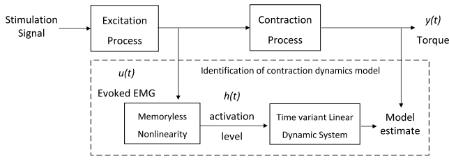
Fig. 4. Muscle model structure. The present work focuses on the contraction dynamics model contained in the rectangle within the dashed line. The memoryless nonlinearity is modeled by an n th-order polynomial function. The linear dynamics is chosen as an ARX model.
