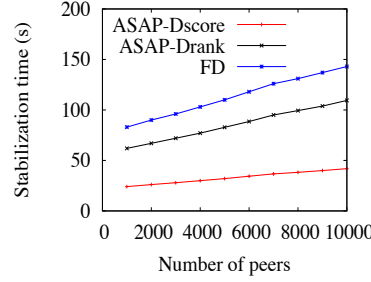
(b) Stabilization time vs. Number of peers.
