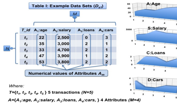
Fig. 1. Notations of a Data Set.
