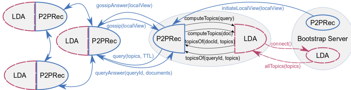
Figure 1: P2Prec Architecture
