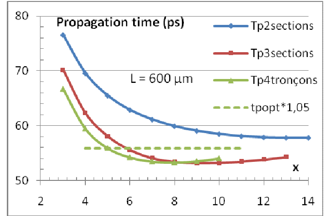
Fig. 5b: Variation of the propagation time versus the multiplying factor of the buffer's width for different configurations. L = 600 μm
