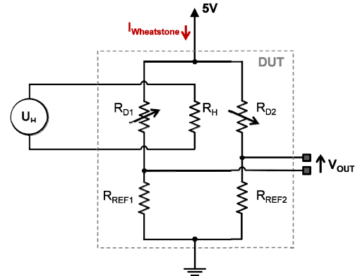
Figure 7. Electrical test setup
