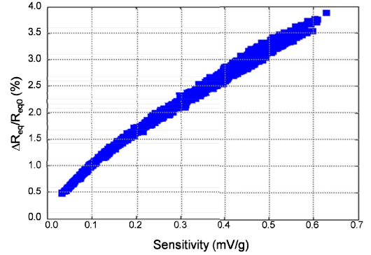
Figure 6. Relative deviation of Wheatstone bridge's equivalent impedance ( \Delta R_{eq} / R_{eq0} ) vs. device sensitivity
