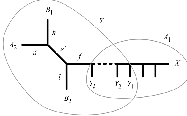
FIGURE S2. Illustration for the proof of Lemma 13.
