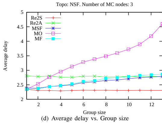
Fig. 15. Performance of algorithms vs. Group size in NSF network with 3 random MC nodes
