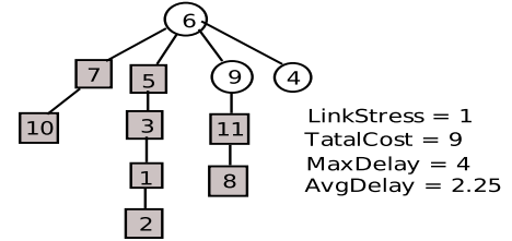
Fig. 8. Member-First with New Priority Definition light-forest
