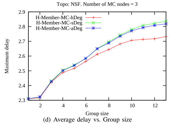
Fig. 4. H-Member-MC-sDeg, H-Member-MC-hDeg and H-Member-MC-aDeg when Group size varies in NSF network with 3 random MC nodes
