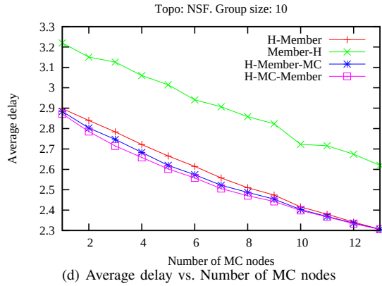
Fig. 3. H-Member vs. Member-H and Member-MC vs. MC-Member when Number of MC nodes varies in NSF network with group size of 10
