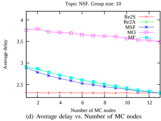
Fig. 17. Performance of algorithms vs. Number of MC nodes in NSF network with group size of 10
