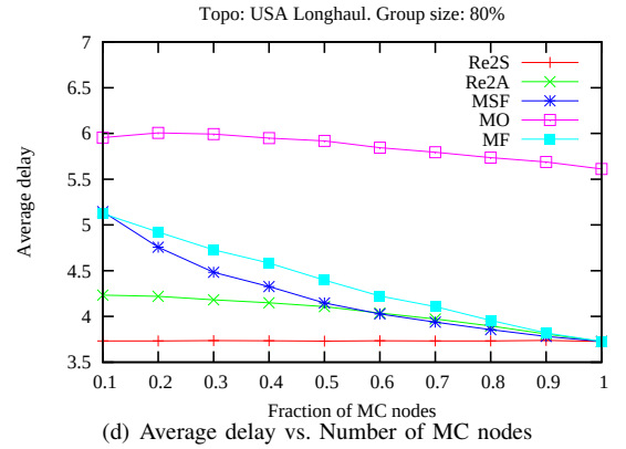
Fig. 18. Performance of algorithms vs. Number of MC nodes in USA Longhaul network with group size of 80%
