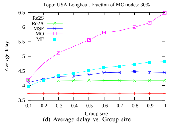
Fig. 16. Performance of algorithms vs. Group size in USA Longhaul network with 30% random MC nodes
