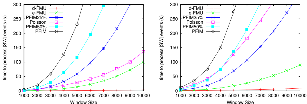
FIGURE 10. Processing time for |SW| events with increasing size of SW on synthetic (top) and accident (bottom) datasets
