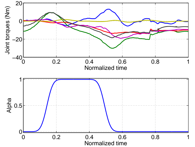
Figure 5: Typical joint torques at the joints of the avatar (chest joint and right arm joints). The torque references sent to the actuators of the robot are smooth even when the value of the homotopy variable changes.
