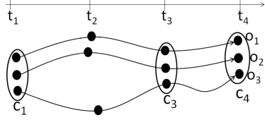
Fig. 3. An example of closed swarm.
