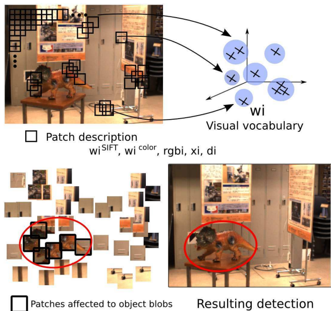
Fig. 6. First row: patches are extracted in a very dense manner. Each patch is associated to the closest visual word for sift and color descriptors, and then represented by the words indexes (w_i^{SIFT}, w_i^{color}) , a RGB value (rgb_i) , a position (x_i) and a depth (d_i) given by the disparity map. Second row: the model computes the best assignment of patches to object blobs or background and estimates to blobs positions.
