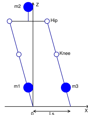
Fig. 4. Illustration of 3MLIPM in the frontal plane
