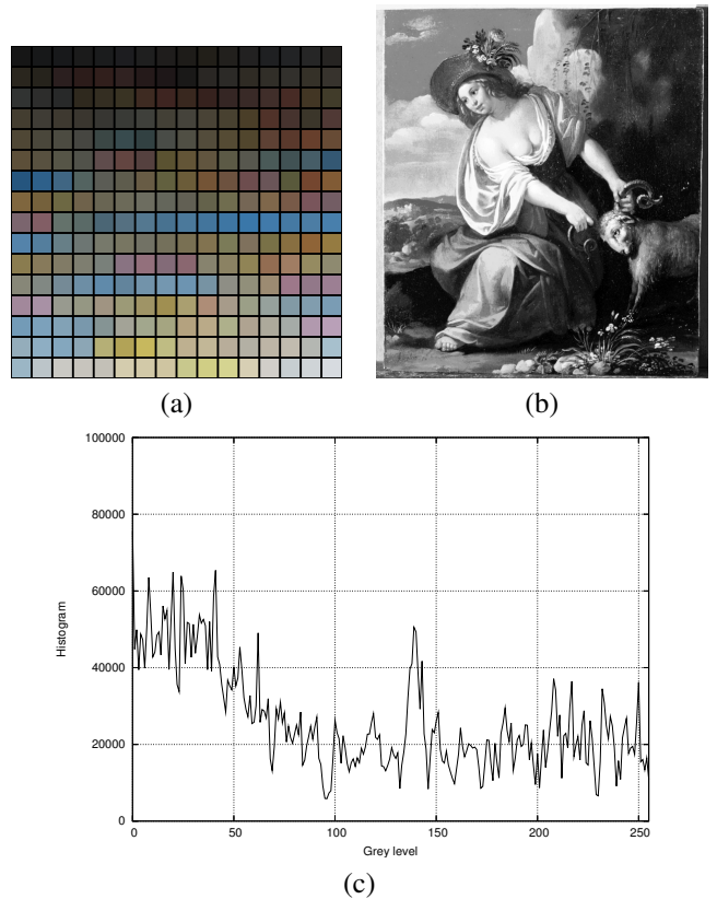
Figure 5: Application of the layer scanning algorithm (with K = 256 colors): a) Color Palette after the color reordering, b) Index image after the color reordering, c) Histogram of the index image (b).
