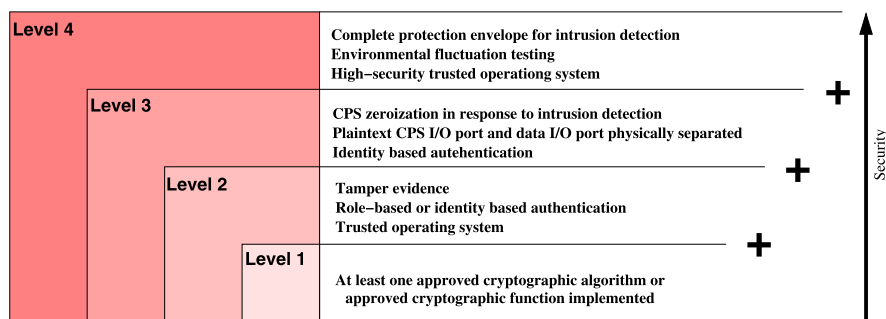
Fig. 2.5 Security requirements in four security levels, according to the FIPS 140-2 Standard
