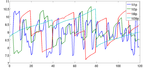
Fig. 3. Evolution of the PSNR of the encrypted video of mobile as a function of the GOP length. Blue: GOP with 1 intra frame and 1 inter frame. Cyan: GOP with 1 intra frame and 39 inter frames.
